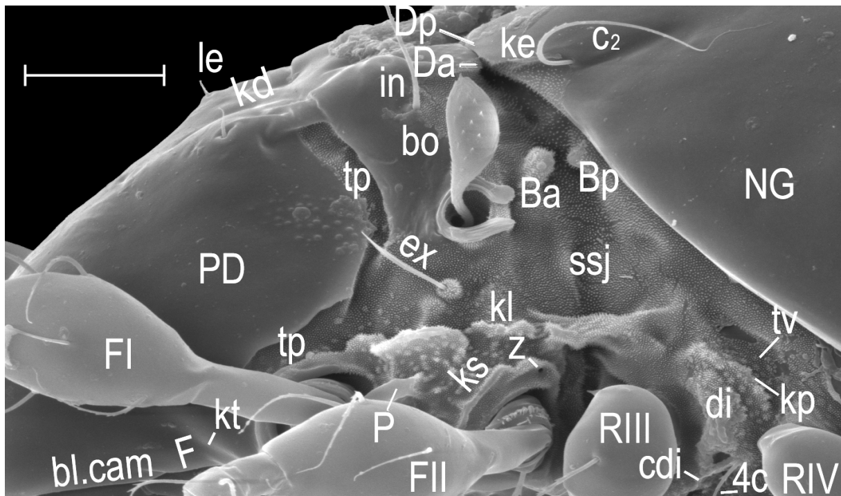
Fig. 2. – Hypogeoppia belgicae n. sp. – Scanning electron micrograph of the anterior part of the body laterally orientated; left side of an animal a bit inclined to the left. The prodorsum (PD), the notogaster (NG) and the legs are partially seen. The prodolateral prominence P is almost completely hidden. FI , FII , femur of the legs I and II. RIII , RIV , trochanter of the legs III and IV. Scale bar, 20 \mu m.
