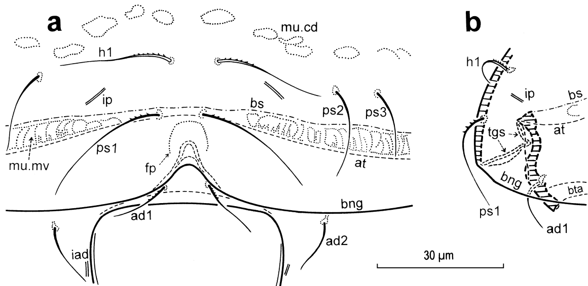
Fig. 3. – Hypogeoppia belgicae n. sp., female. – Posterior parts of the notogaster and ventral shield in a contracted animal, partial, with the anal valves removed. – a, seen from the back. Lines (broken) of apparent outline in the median, posterior fold of the articular cuticle tgs of dorsoventral connection are shown through the cuticle of the notogaster. The part of tgs which turns beyond the fold towards the line at of attachment to the ventral shield and emerges from the postanal fossa (its border is indicated by the dotted line fp ), is not distinguishable in this orientation. mu.mv , marginoventral alignment of insertions of dorsoventral, opisthosomatic muscles – b, right lateral. The horizontal hatching represents an optical section of the tegument passing through the plane of symmetry. bs , border of the ventral shield.
