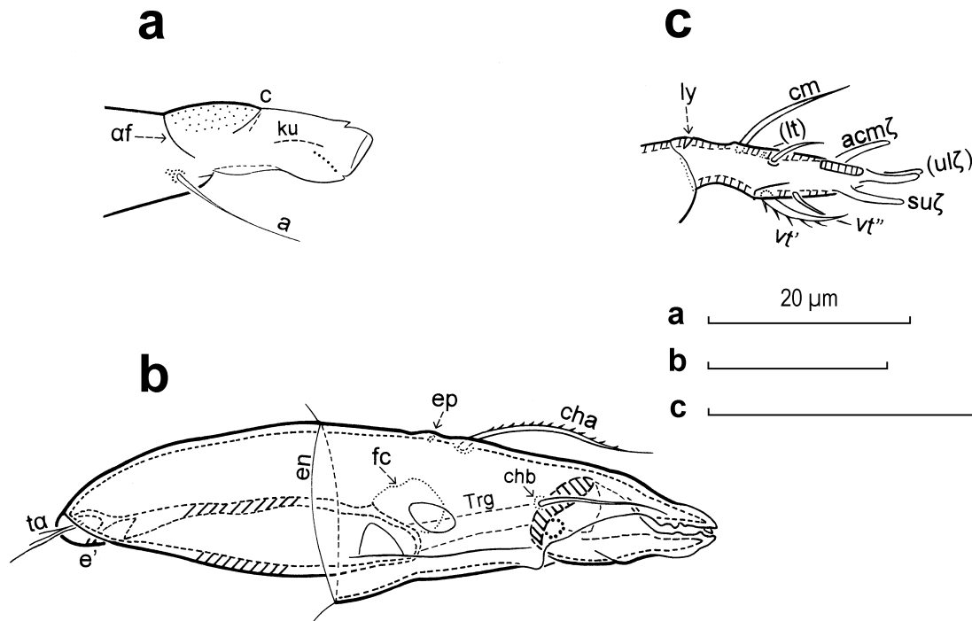
Fig. 5. – Hypogeoppia belgicae n. sp., female. – a, right rutellum, seen laterally, with a part of the gena. The dots below the line ku depict the base of barbs of the comb on the adaxial side of the rutellum seen through the cuticle. The labrum and the lateral lips are not represented. c , collar of the rutellum – b, right chelicera, separated and seen laterally. Only the proximal part of Trägårdh's organ Trg is shown. The part of the chelicera behind the line of attachment en of the cheliceral sheath is inside the body. It is represented as if it is exposed. In this orientation, the dorsal adaxial spine is hidden by the abaxial spine ep which is the only spine to be shown through the dorsal cuticle. The weakly undulating line behind the movable digit marks a longitudinal carina on the abaxial side of the cheliceral body. The hatching directed to the left covers the posterior, more coloured part of the movable digit. The hatching directed to the right indicates partially the base border of the cheliceral body. – c, tarsus of the right pedipalp seen laterally. The solenidion \omega is vertically hatched. The oblique hatching marks an optical section of the tegument through the plane of pseudosymmetry of the segment. cm , culminal seta. su , subultimal eupathidium.
