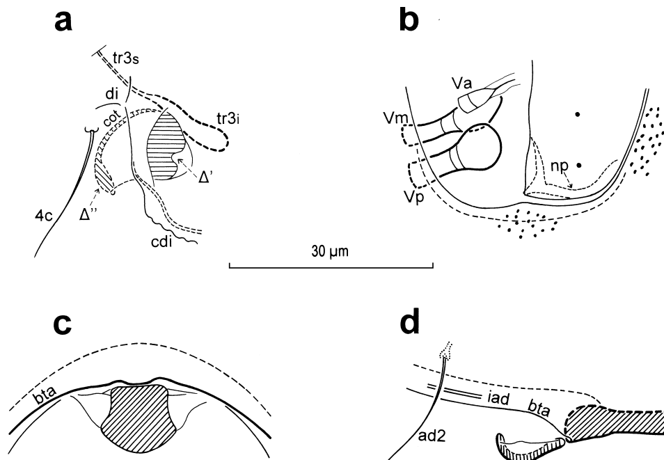
Fig. 4. – Hypogeoppia belgicae n. sp. – a, male, right trachea III, partial, and acetabulum III seen through the cuticle in a dissected fragment of the podosoma. The hind leg is on the left. The horizontal hatching marks the circumtrochanteral opening of the leg III. The oblique hatching represents an optical section of the cotyloid wall III cot and the posterior tooth \Delta'' of the trochanter III-podosoma articulation. – b, female, genital region, partial, in ventral projection, with the right genital valve removed so as to have a direct sight at the genital papillae. A part of the median papilla Vm is not represented in order to completely show the small papilla Va . The papillae are invaginated in their sheath. The sheath of papilla Va is pointed out by two lines of apparent outline whereas the sheath of papillae Vm and Vp are not discernible. The dots indicate the base of the two posterior genital setae. The granulation laterad and behind the circumgenital opening is partially shown. np , posterior, internal nervure of the genital valve. – c, male, preanal organ (hatched) in ventral projection after the removal of anal valves. The organ is almost horizontal. It has remained near the border of the circumanal opening. – d, same organ (vertically hatched) in lateral view. The gnathosoma is on the right. The oblique hatching represents an optical section of the cuticle passing through the plane of symmetry.
