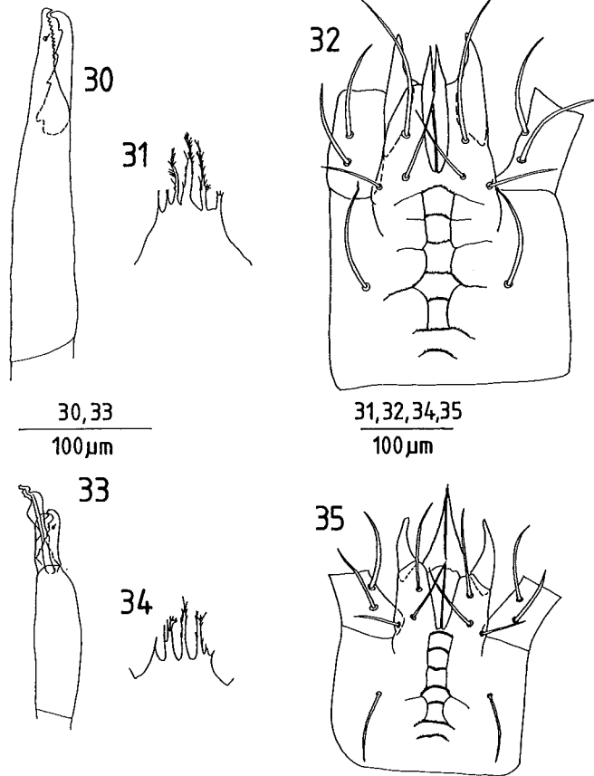
Figs 30–35. Lasioseius peterfuldi sp. nov.: Figs 30–32: Holotype female. (30) chelicera, (31) tectum, (32) subcapitulum. Figs 33–35: Paratype male. (33) chelicera, (34) tectum, (35) subcapitulum.
