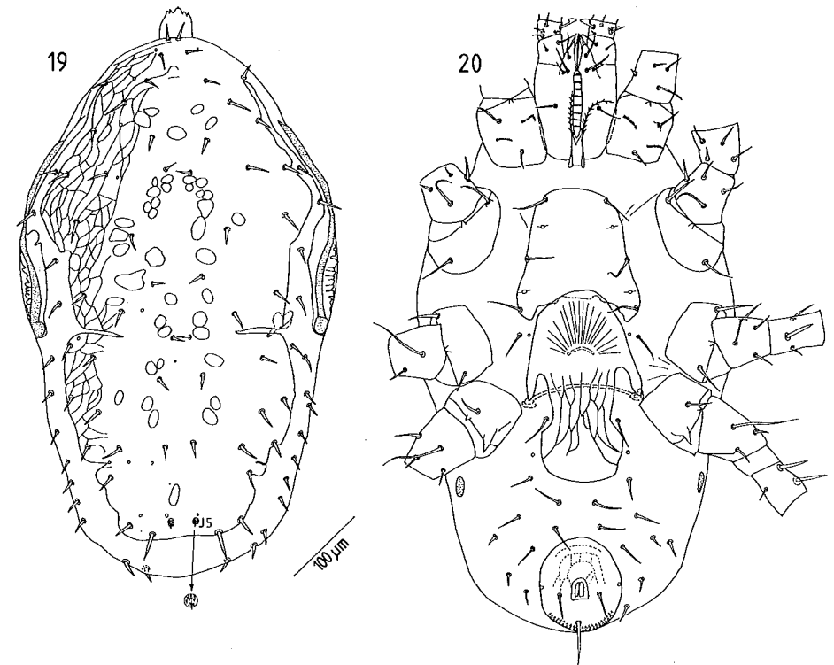
FIGS 19–20. Rhinoseius panamensis Fain, Hyland and Aitken, 1977, female: (19) body dorsum, (20) body venter.
