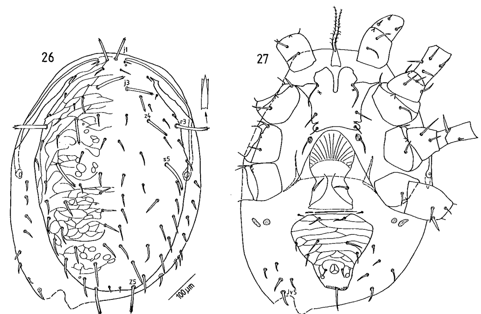
FIGS 26–27. Lasioseius peterfuldi sp. nov., Holotype female: (26) body dorsum, (27) body venter.
