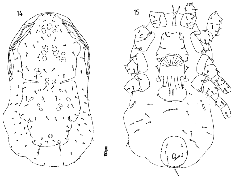
FIGS 14–15. Rhinoseius haplophaedia sp. nov., Holotype female: (14) body dorsum, (15) body venter.
