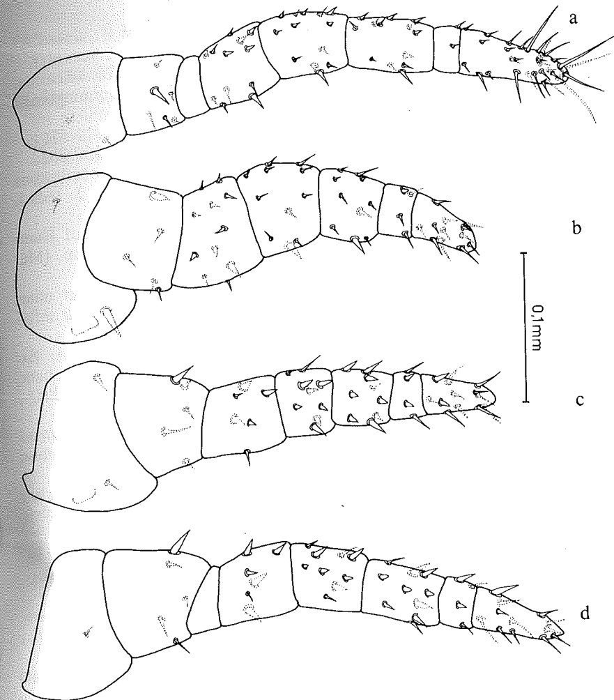
Fig. 24. Rhinoseius perezgloriae sp. n. legs I to IV in the female (a,b,c,d).
