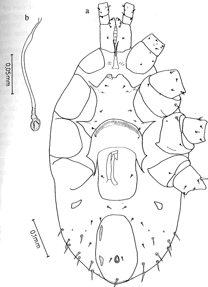
Fig. 23. Rhinoseius perezgloriae sp. n. female in ventral view (a), inseminating organ (b).
