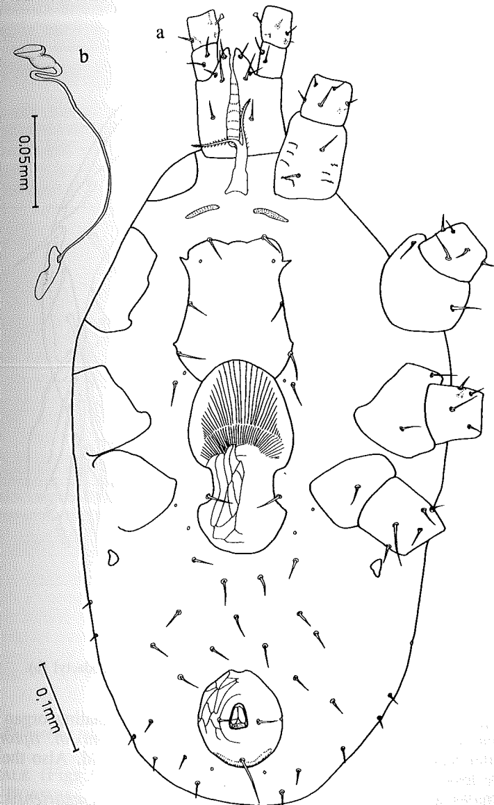
Fig. 7. Rhinoseius pastora sp. n. female in ventral view (a), inseminating organ (b).
