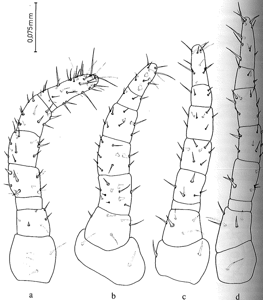
Fig. 12. Rhinoseius nadachowskyi sp. n. legs I to IV in the male (a,b,c,d).
