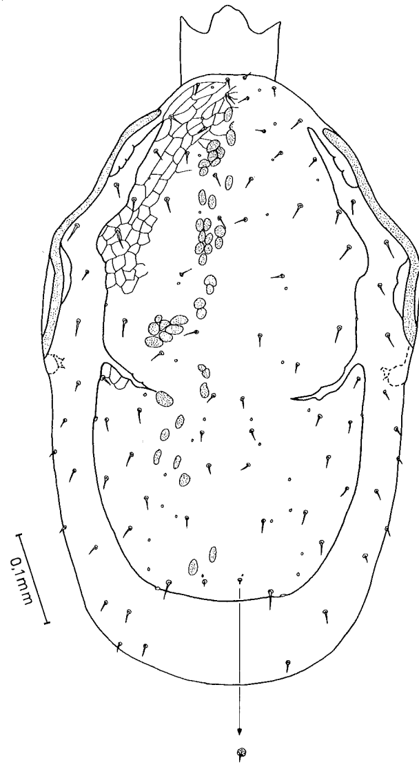
Fig. 6. Rhinoseius pastora sp. n. female in dorsal view.
