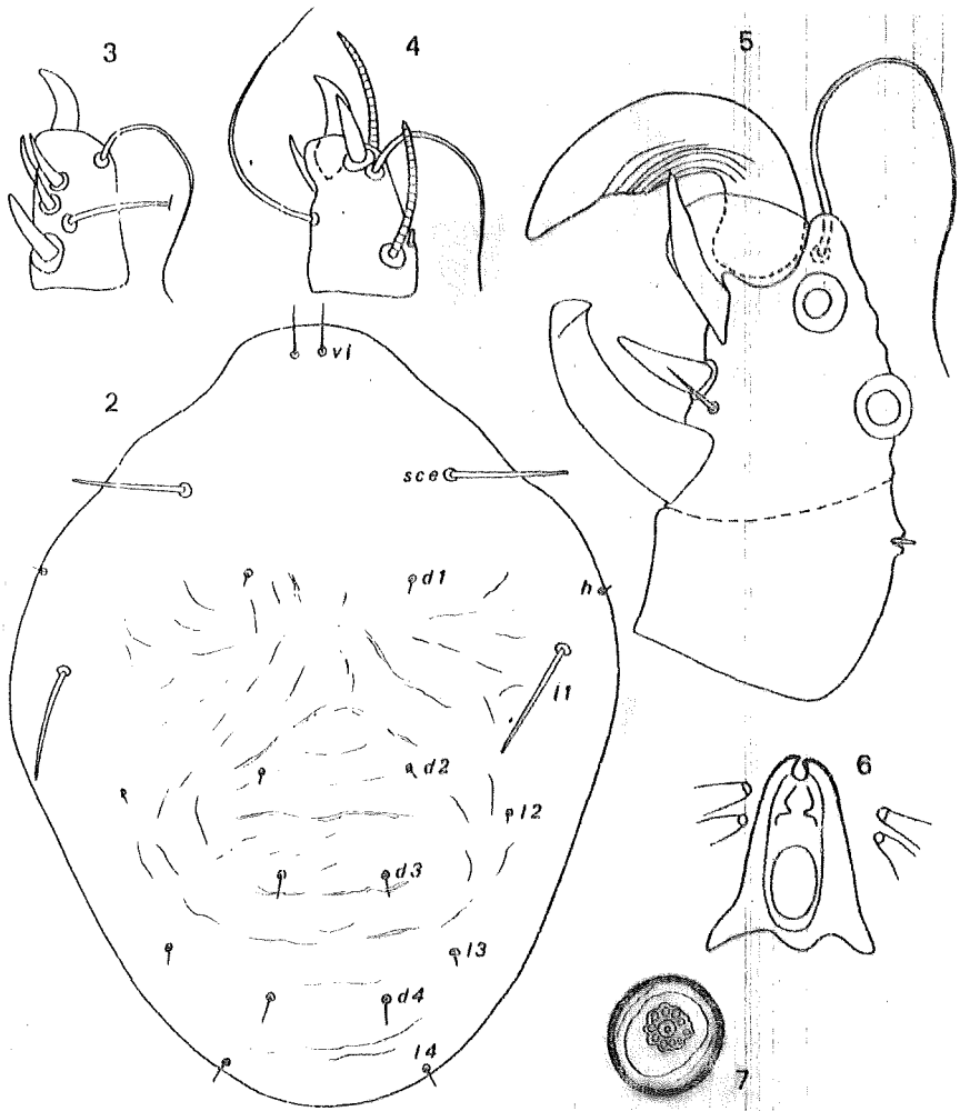
Fig. 2-7. — Askinasia antillarum sp. n., Male: (2), in dorsal view; (3), tarsus I in ventral view; (4), tarsus I in dorsal view; (5), tibio-tarsus IV, posterior surface; (6), genital organ; (7), adanal sucker.
