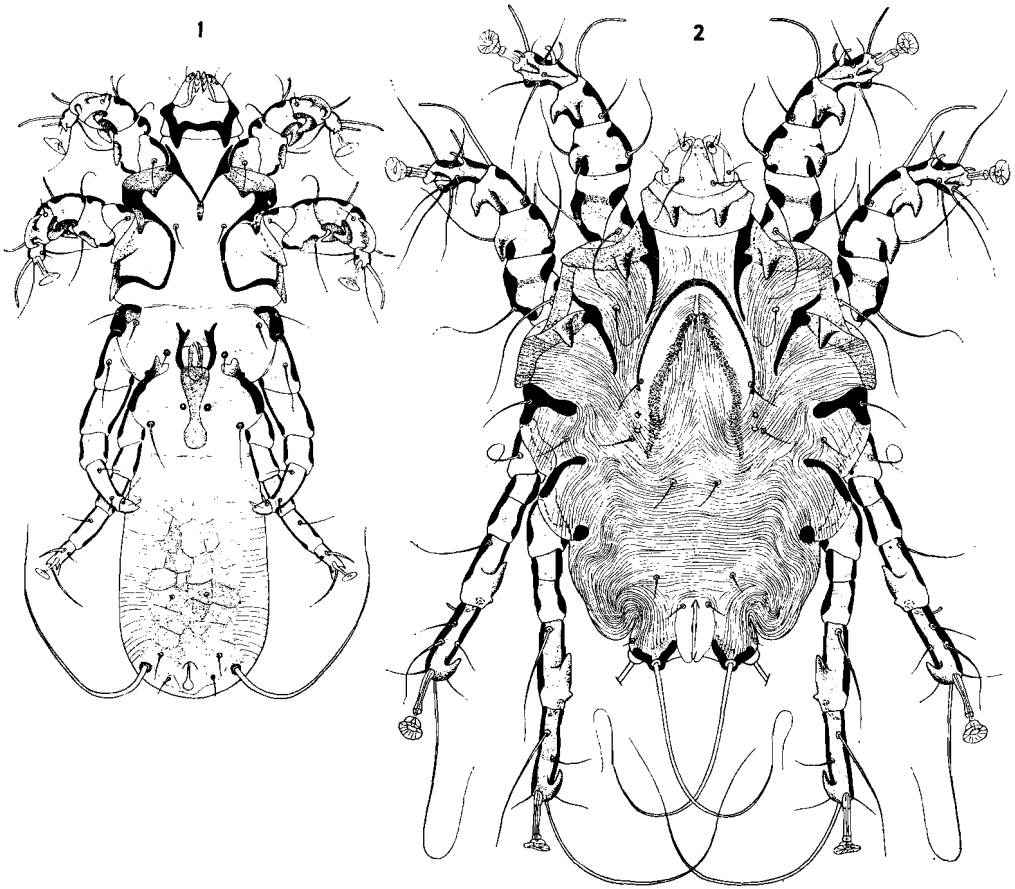
FIG. 1-2 : Examples of attaching organs on the idiosoma, the gnathosoma and the legs in the male of Galagalges congolensis Fain (Galalgidae) (fig. 1) and in the female of Gaudalgies caparti Fain (Psoroptidae) (fig. 2).
