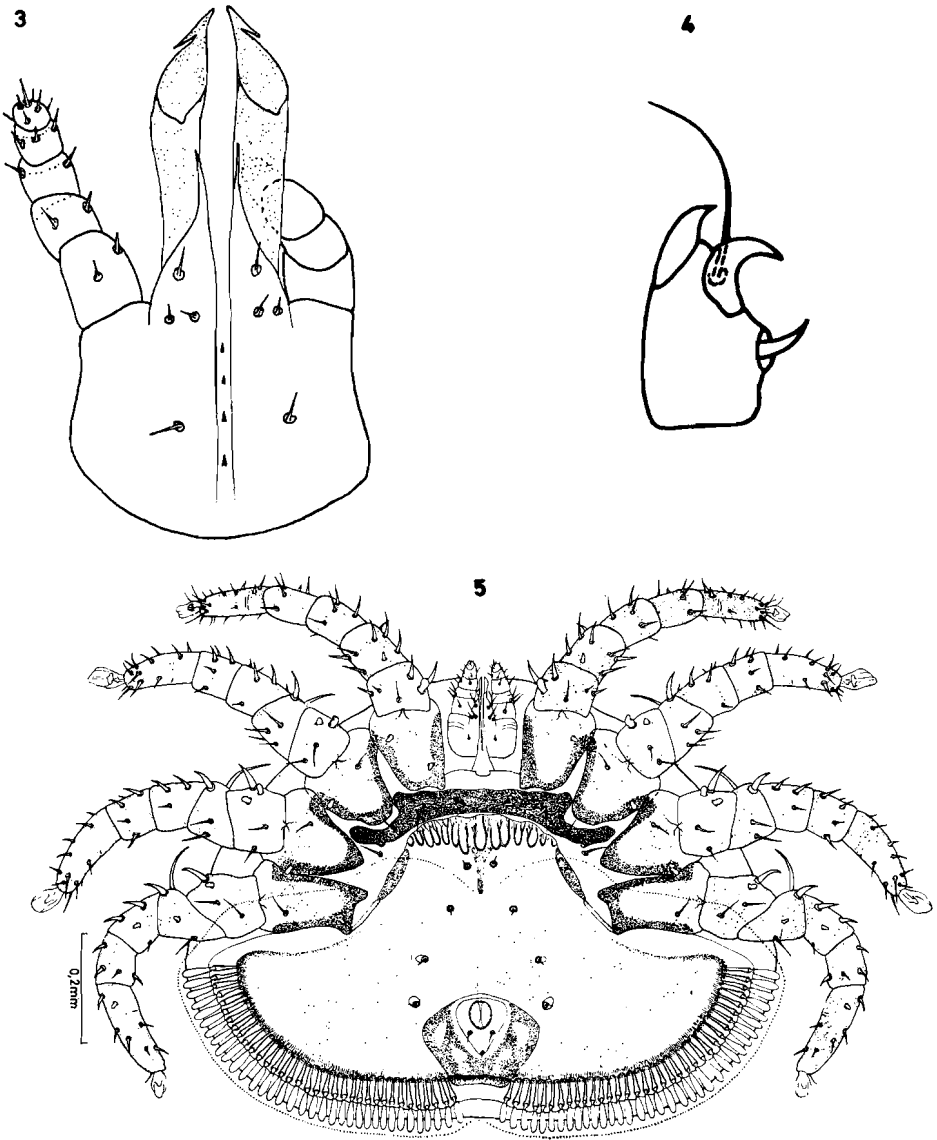
FIG. 3-5 : Strongly elongate and barbed corniculi in Ixodorhynchus fonsecae Fain (Ixodorhynchinae) (fig. 3). Tarsus IV in Rodhainyssus yunkerii Fain (Gastronyssidae) showing the small pincer-like organ (fig. 4). Transversal elongation of the body in the female of Omentolaelaps mehelyae Fain (Omentolaelapidae) (fig. 5).
