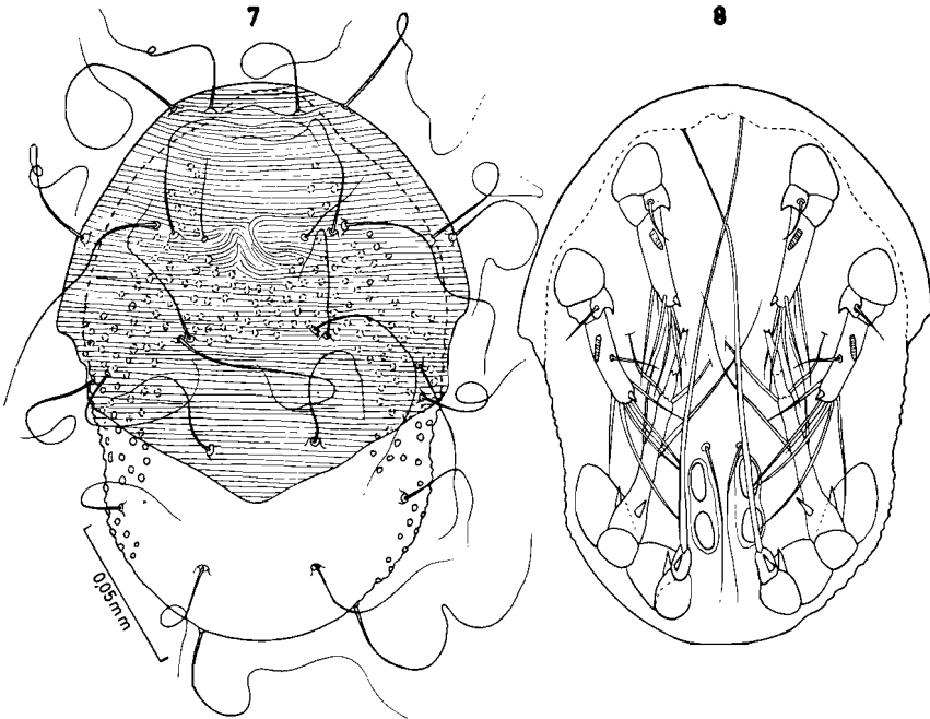
FIG. 6-8 : Small hypopus of Hypodectes propus (Nitzsch) found free in the nest of Columba palumbus , in Belgium (fig. 6). Egg found free in the same nest, the chitinous layer has disappeared, the striate-hairy membrane is the vestige of the larval stage, the verrucous membrane being the vestige of the protonymphal stage (fig. 7). The same egg showing the hypopus that it contains (fig. 8).
