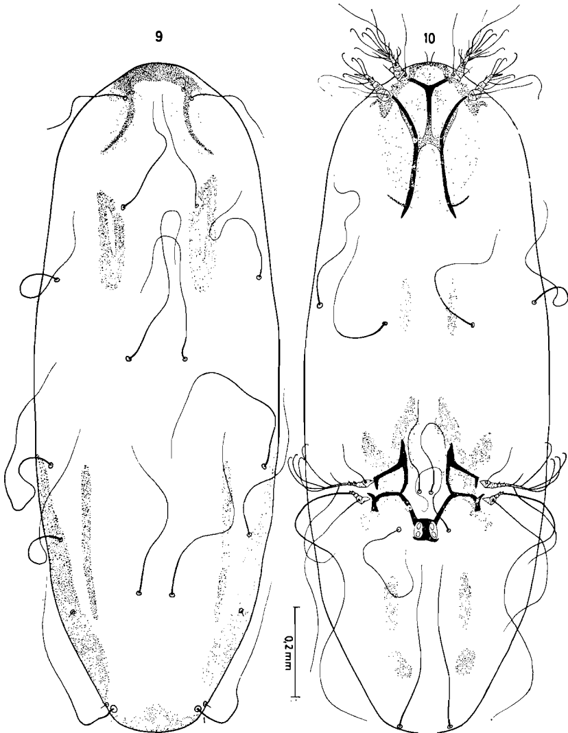
FIG. 9-10 : Large hypopus of Hypodectes propus (Nitzsch) found in the subcutaneous tissues of Columba palumbus in Belgium.
